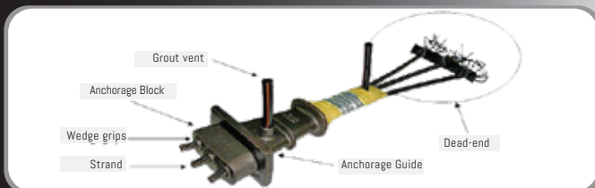
LIVE END ANCHORAGE
